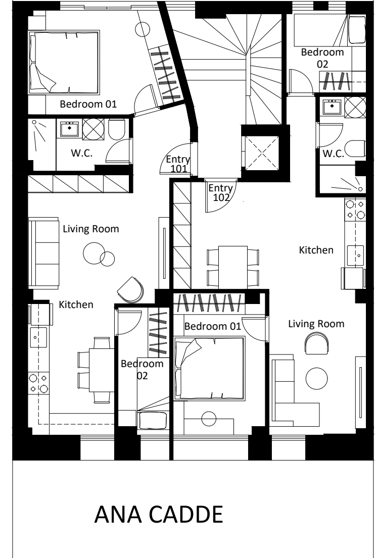
BUILDING A_FIRST FLOOR PLAN
