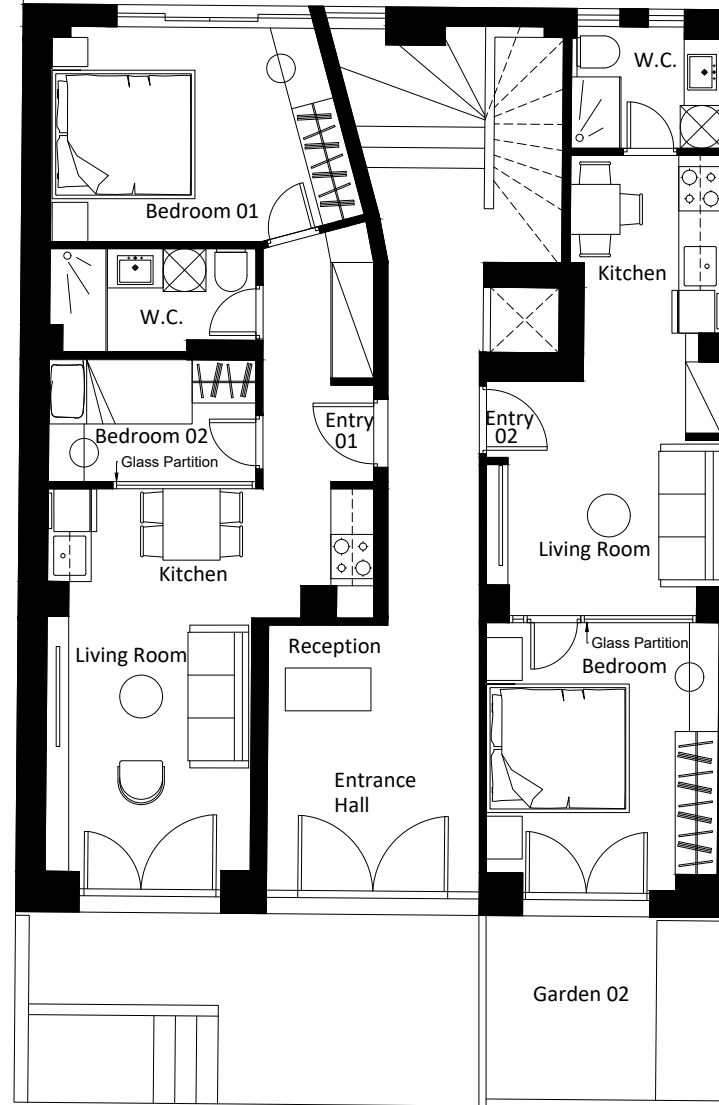
BUILDING B_GROUND FLOOR PLAN
